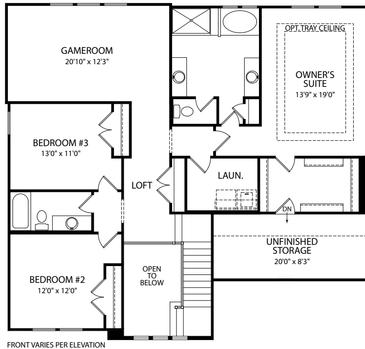
Second Level
