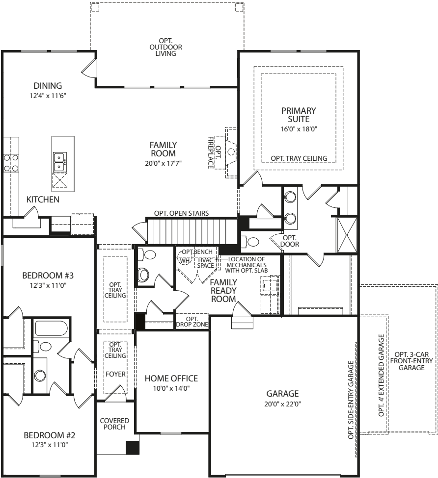
Main Level
