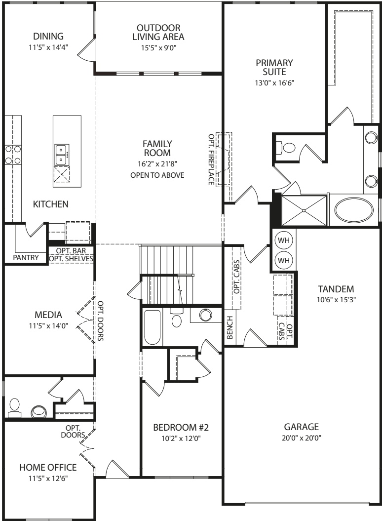
Main Level
