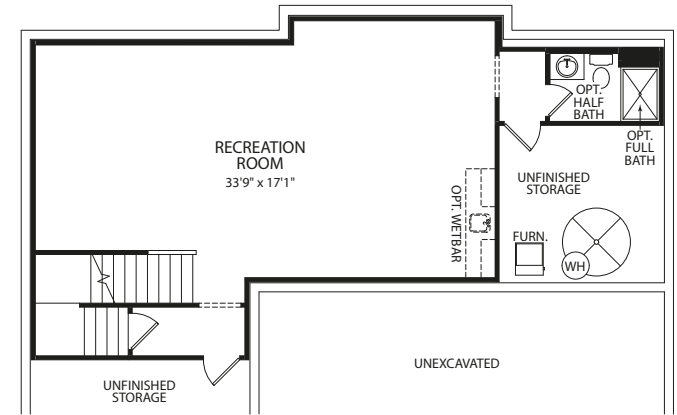
Optional Finished Lower Level
