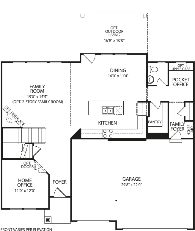
Main Level
