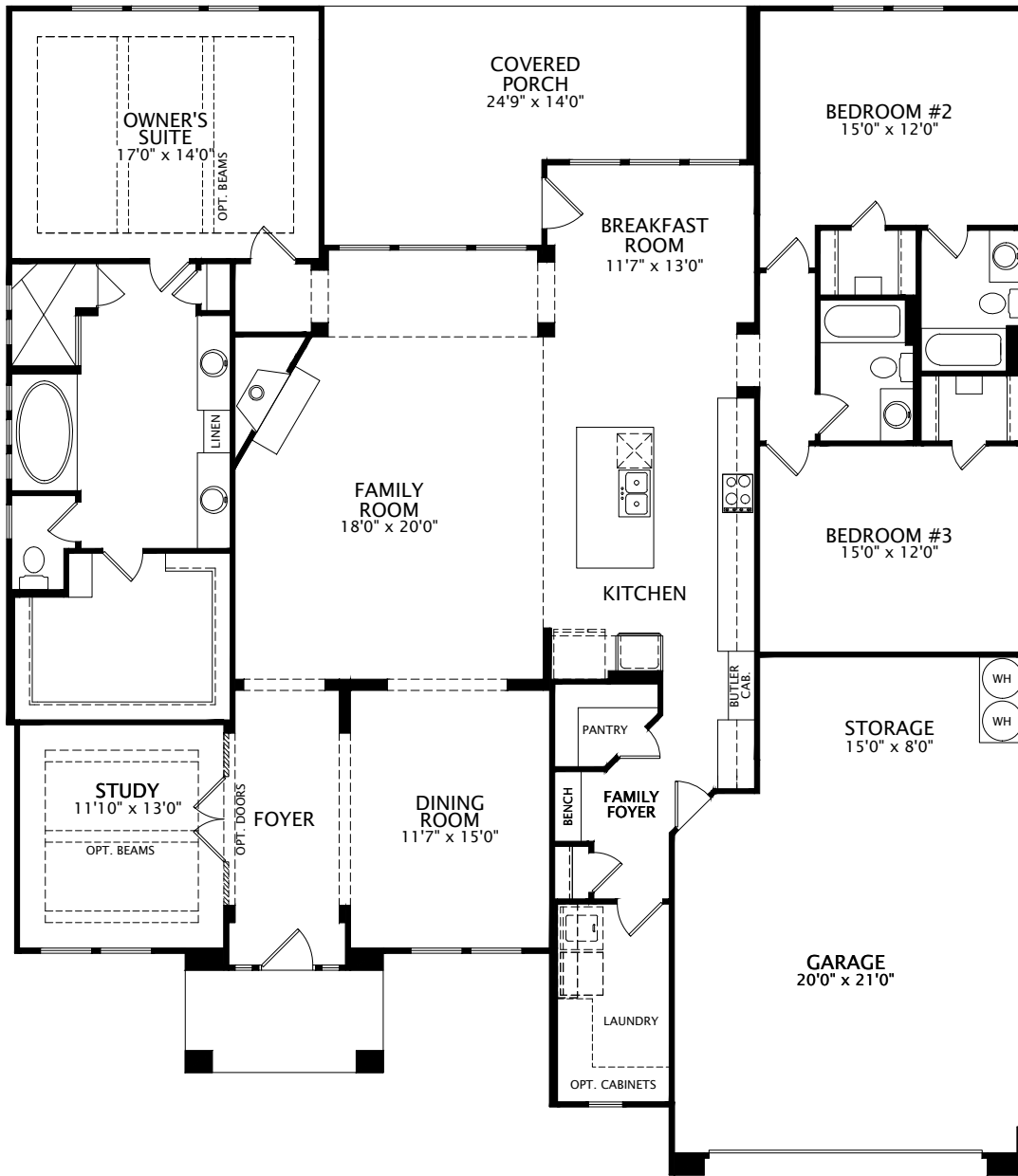
Main Level FRONT VARIES PER ELEVATION
